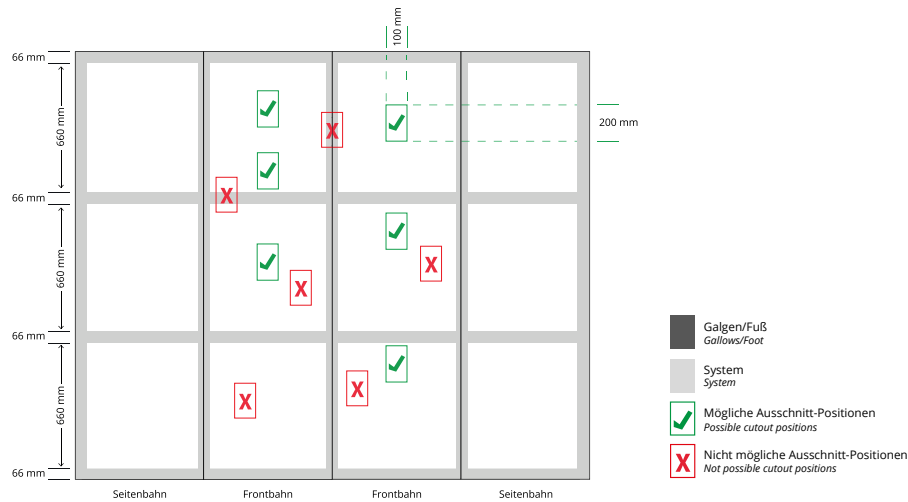
Frontansicht Front view
